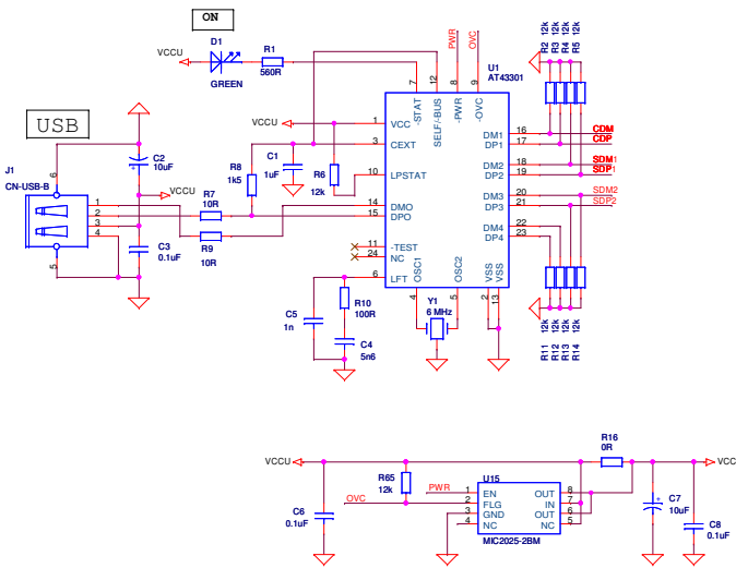
RE Standard 1.2: USB hub, power key, connectors Rig Expert Ukraine Ltd.
